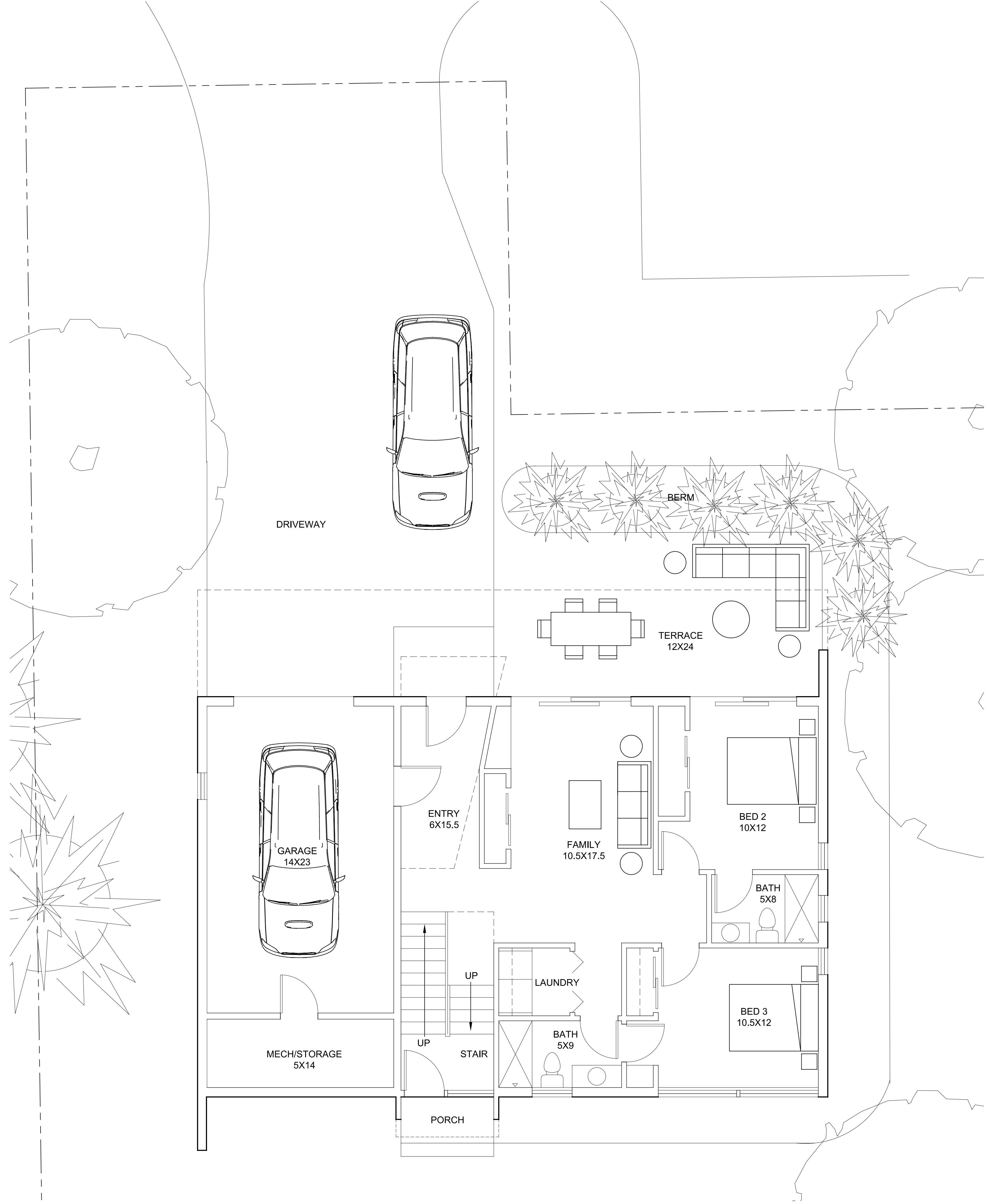
GROUND LEVEL PLAN 1/4"=1'-0"
